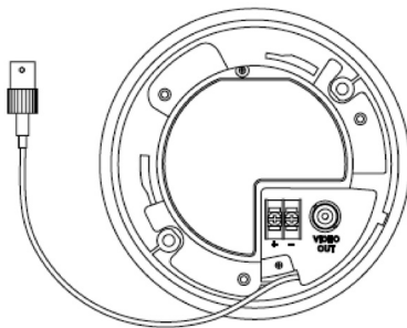
Rear View of Dome Base
