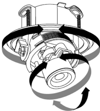
3-Axis Gimbal (Shown Here with Ceiling Mount)
